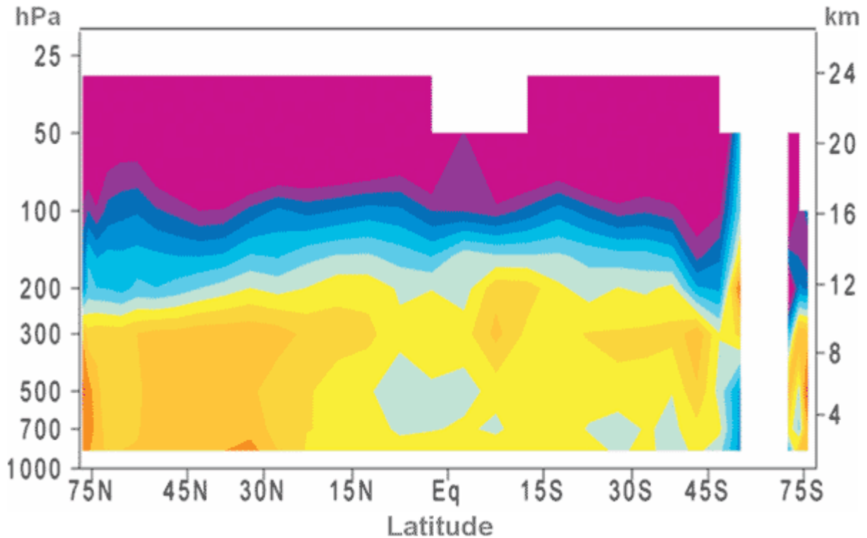
Altitude-vs.-latitude plot of observed relative warming rates in the satellite era. The greater rate of warming in the tropical mid-troposphere that is projected by general-circulation models is absent in this and all other observational datasets, whether satellite or radiosonde. Altitude units are hPa (left) and km (right). Source: Hadley Centre for Forecasting (HadAT, 2006).
