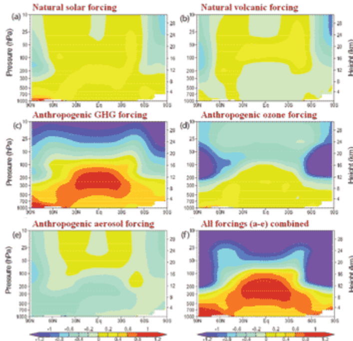
Modeled zonal mean atmospheric temperature change (°C per century, 1890-1999) in response to five distinct forcings (a-e), and to all five forcings combined (f). Altitude is in hPa (left scale) vs. latitude (abscissa). Source: IPCC (2007).
